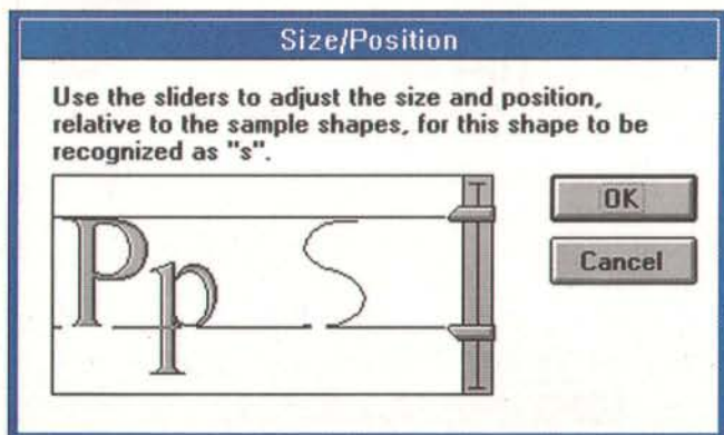
Screen 7: Specifying a shape's size and its position relative to a baseline helps resolve ambiguity.
